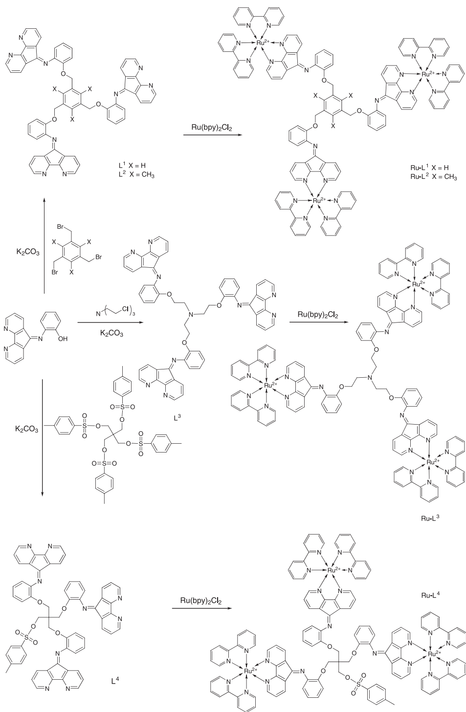
Scheme 1. Synthesis of tripodal ligands L^{1-4} and corresponding Ru(II) complexes Ru-L^{1-4} .
