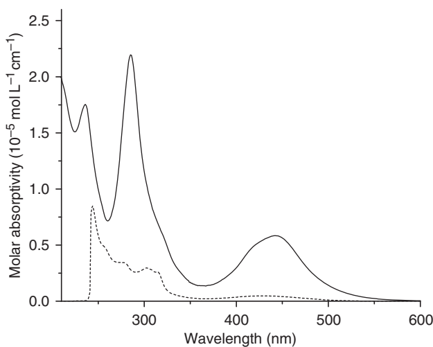
Figure 1. Absorption spectra of Ru-L 1 (10 -5 mol L -1 , (—), typical for Ru-L 1-4 ) in MeCN and L 1 (10 -5 mol L -1 , (---), typical for L 1-4 ) in CHCl 3 solution.
